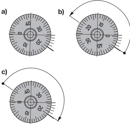
Type DIN911
